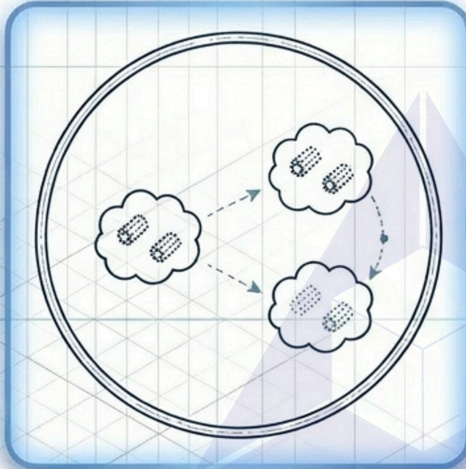
1. Replication
