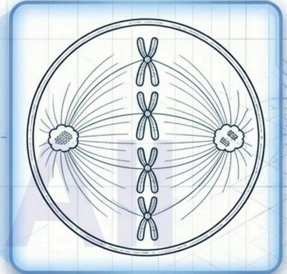
3. Spindle Formation
